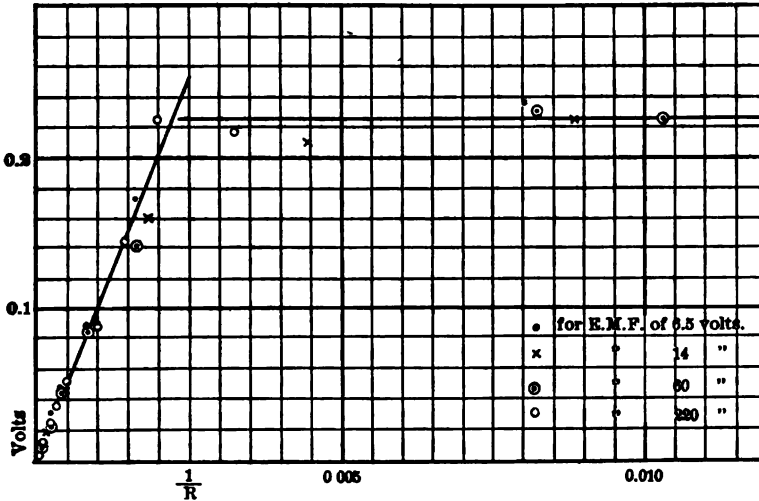
DIAGRAM SHOWING RELATIONS BETWEEN VOLTAGE AND CONDUCTANCE.
