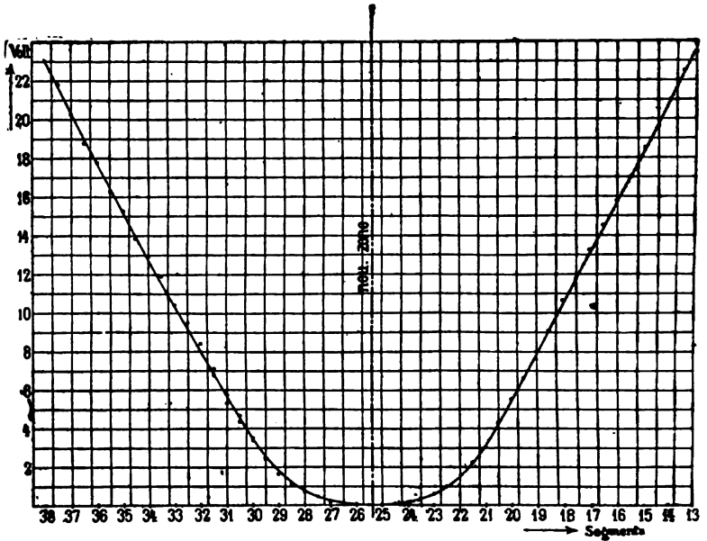
FIG. 22. POTENTIAL CURVE OF 10-HP SHUNT MOTOR IN NEUTRAL ZONE, THE BRUSHES BEING REMOVED.
