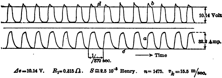
FIG. 32. VERY SLIGHT SPARKING.
