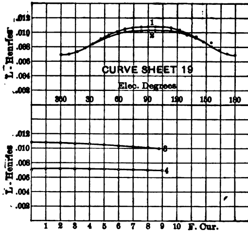
CURVE SHEET 19.—REACTANCE CURVES.
