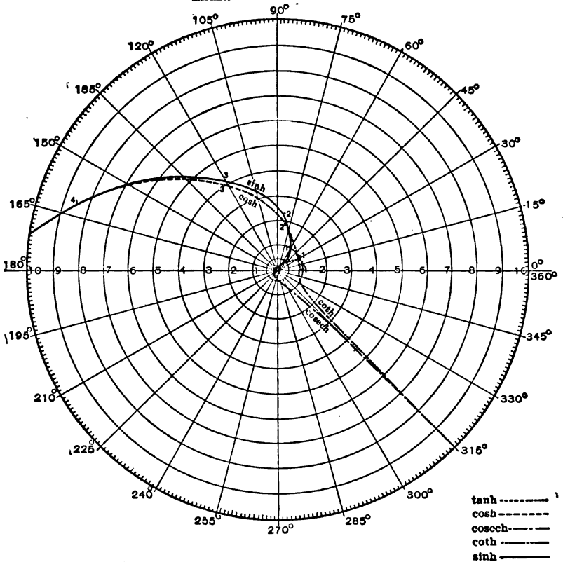
FIG. 13.—LOCI OF \sinh , \cosh , \tanh , \coth AND \operatorname{cosech} x / 45^\circ BETWEEN THE LIMITS OF 0 AND 10 OF THE RESULT.
