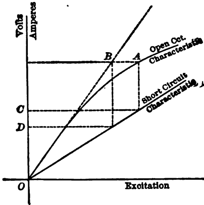
FIG. 1.—NO-LOAD AND SHORT-CIRCUIT CHARACTERISTICS.
