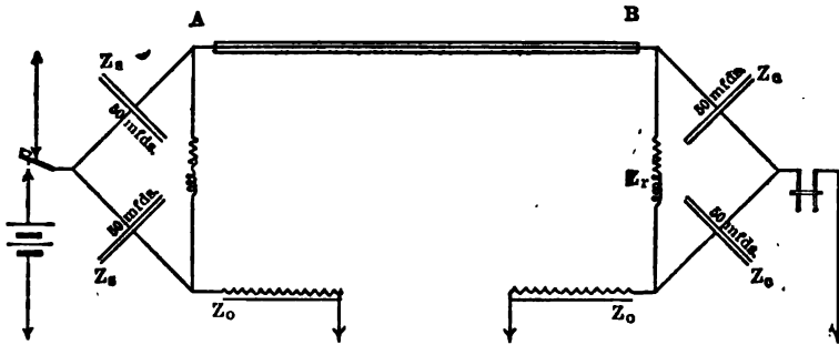
FIG. 6.—CONDENSER OF 50 MICROFARADS AT EACH END AND CABLE DUPLEXED.
