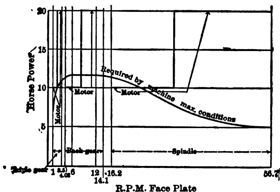
FIG. 12.— DATA RELATIVE TO EDISON THREE-WIRE MOTOR EQUIPMENT FOR LATHE, A.-B.-COMPANY.
