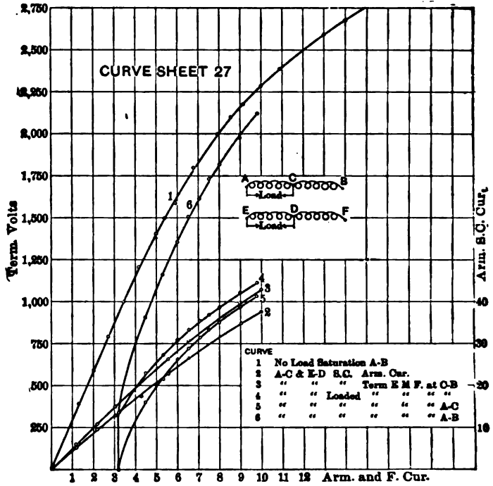
CURVE SHEET 27.—LOAD SATURATION AND SHORT-CIRCUIT CURVES. 65 kw, 2-ph, 2400 volts, 60 p.p.s., 900 r.p.m., .280" air-gap. One side only of generator loaded @ 13.5 Amps.
