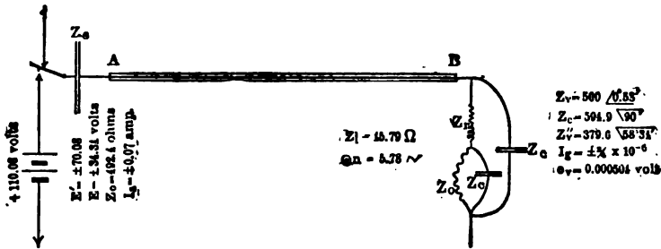
FIG. 12.—EQUIVALENT SIMPLEX CONNECTIONS OF DUPLEX SYSTEM SHOWN IN FIG. 6.
