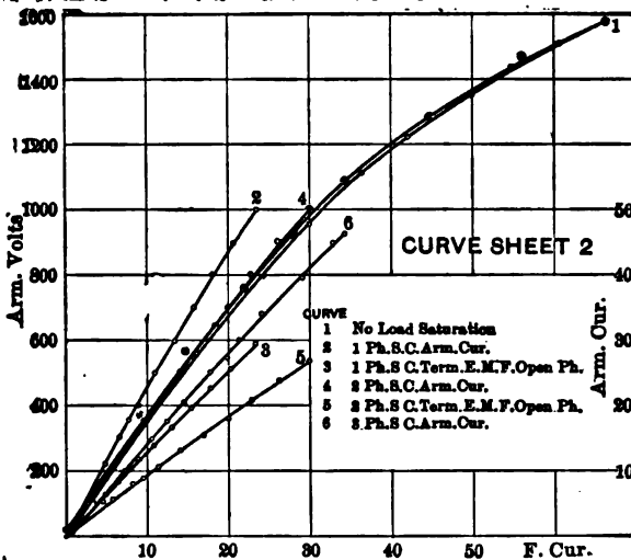
CURVE SHEET 2.—SHORT CIRCUIT AND SATURATION CURVES. 70 kw, 3-ph, 2300 volts Y. 60 p.p.s., 276 r.p.m., .2525" air-gap.
