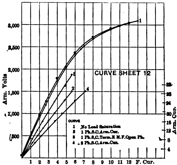
CURVE SHEET 12.— SHORT-CIRCUIT AND SATURATION CURVES. 65 kw, 2-ph, 2400 volts, 60 p.p.s., 900 r.p.m., .148" air-gap.
