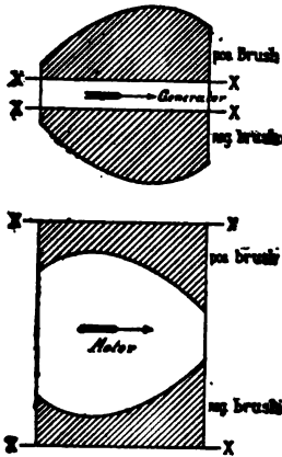
FIGS. 18b AND 18c. POTENTIAL CURVES UNDER THE BRUSHES OF A GENERATOR AND MOTOR.
