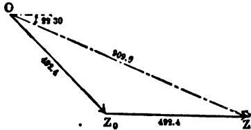
FIG. 10.— IMPEDANCE ( z_o + z_r ) OF CABLE FOR THE FREQUENCY 5.78 ~ AND A RECORDER-COIL OF NO REACTANCE AND BEST RESISTANCE.
