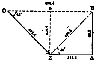
FIG. 11.— IMPEDANCE ( z_o + z_r ) OF CABLE FOR THE FREQUENCY 5.78 ~ AND A RECORDER-COIL OF j 348.2 OHMS REACTANCE AND BEST RESISTANCE.
