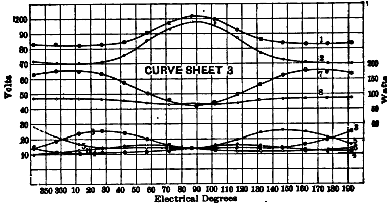
CURVE SHEET 3.— STATIC IMPEDANCE CURVES.
