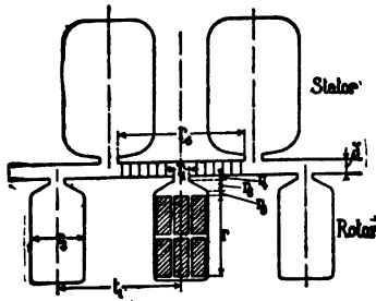
FIG. 51. MOTOR WITH UNIFORMLY DISTRIBUTED STATOR IRON.
