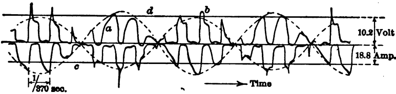
FIG. 50. VERY STRONG SPARKING.
