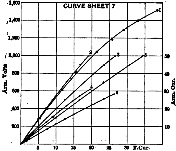
CURVE SHEET 7.—SHORT-CIRCUIT AND SATURATION CURVES. 70 kw, 3-ph, 2300 volts Y. 60 p.p.s., 276 r.p.m., .119" air-gap.
