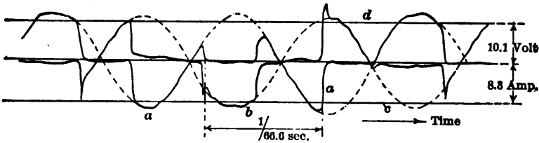
FIG. 49. SLIGHT SPARKING.
