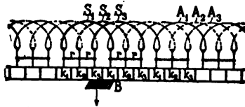
FIG. 62. WINDING WITH RESISTANCE CONNECTIONS.
