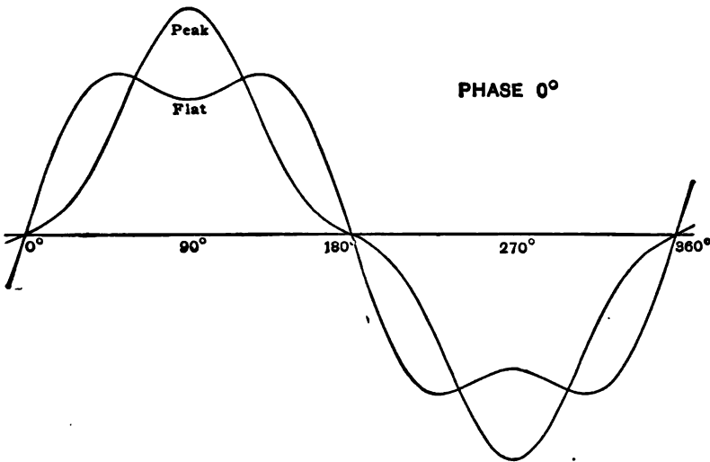
FIG. 1. Showing the resultant of combining with the fundamental a harmonic of three times the frequency, 25 per cent of the magnitude of the fundamental giving, first, a peaked wave and, second (when the phase of the harmonic is reversed), a flat or dimpled wave. Both fundamental and harmonic are of sine wave form.
