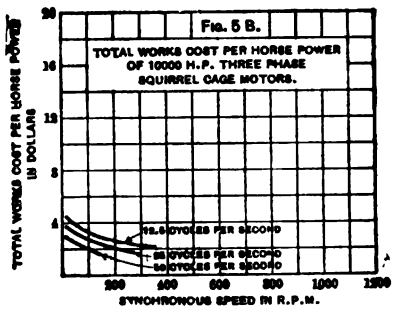
FIG. 5.—RELATION OF COST TO SYNCHRONOUS SPEED.
