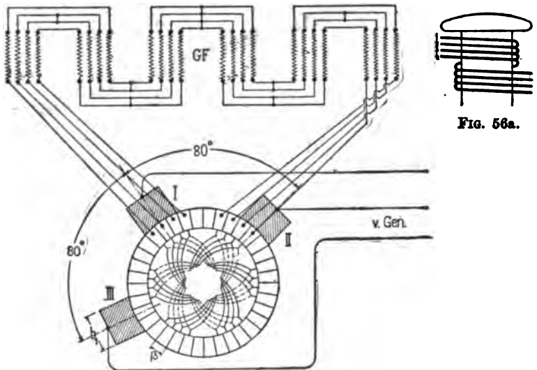
FIG. 56. CONNECTIONS OF HEYLAND COMMUTATOR FOR SELF-EXCITATION OF A SIX-POLE SYNCHRONOUS MACHINE.
