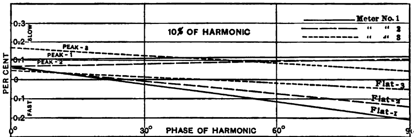
FIG. 6. Showing the variation in the rate of three induction meters with 10 per cent harmonic in the current as the phase of the harmonic is changed from 0 deg. to 90 deg.
