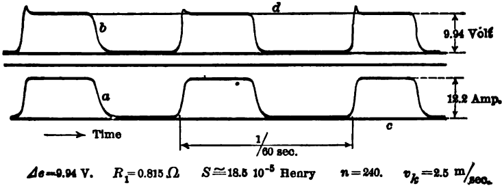
FIG. 33. SLIGHT SPARKING.
