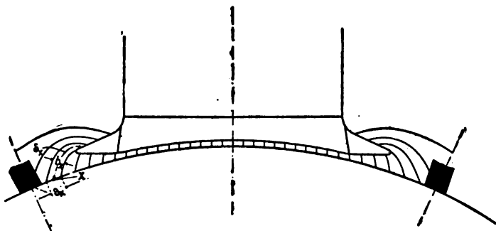
FIG 13. FIELD OF DIRECT-CURRENT SHUNT MACHINE AT NO-LOAD.
