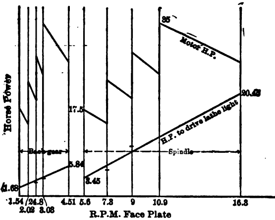
FIG. 13.— DATA RELATIVE TO MOTOR EQUIPMENT FOR LARGE GUN LATHE SHOWING ADVANTAGE OF A CONSTANT TORQUE SYSTEM.
