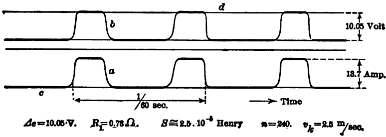
FIG. 31. NO SPARKS WHATEVER.
