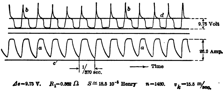
FIG. 34. VERY STRONG SPARKING.
