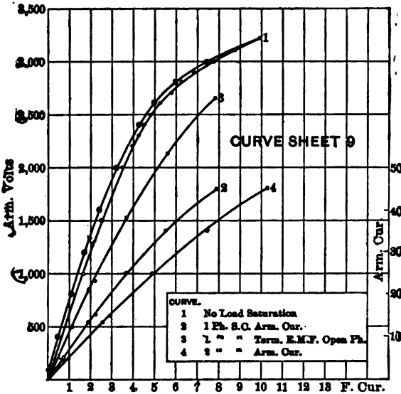
CURVE SHEET 9.—SHORT-CIRCUIT AND SATURATION CURVES.
