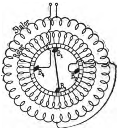
FIG. 55. STATOR AND ROTOR WINDING OF COMPENSATED SINGLE-PHASE MOTOR.
