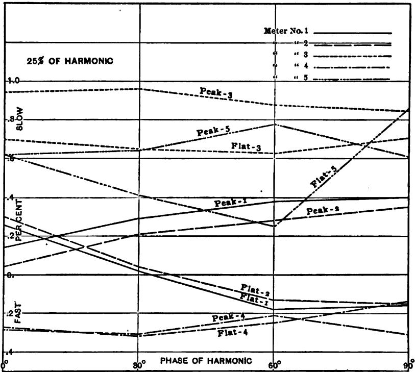
FIG. 5. Showing the variation in the rate of five induction meters with 25 per cent harmonic in the current as the phase of the harmonic is changed from 0 deg. to 30 deg., 60 deg. and 90 deg.
