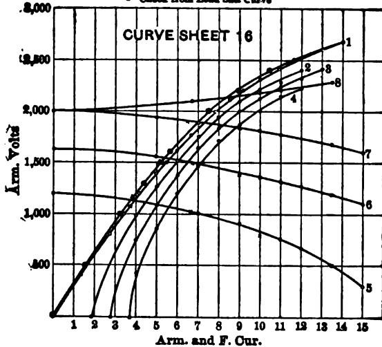
CURVE SHEET 16.—LOAD SATURATION AND REGULATION CURVES. 65 kw, 2-ph, 2400 volts, 60 p.p.s., 900 r.p.m., .280" air-gap.
