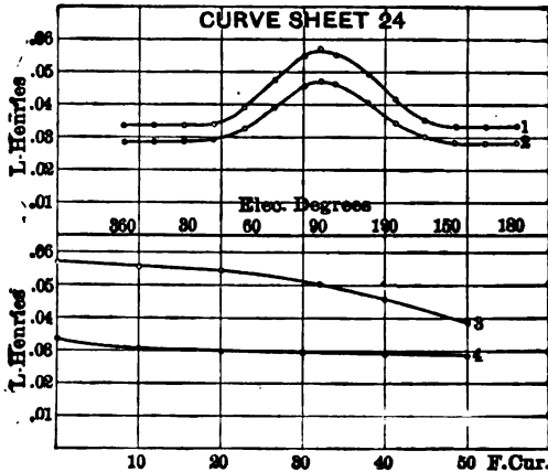
CURVE SHEET 24.—REACTANCE CURVES. 70 kw, 3-ph, 2300 volts Y. 60 p.p.s., 276 r.p.m., .119" air-gap. 6 ampa. @ 60 p.p.s., forced through 1 ph.
