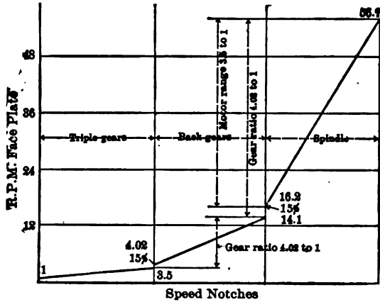
FIG. 10.—LATHE, A.-B.-COMPANY.
