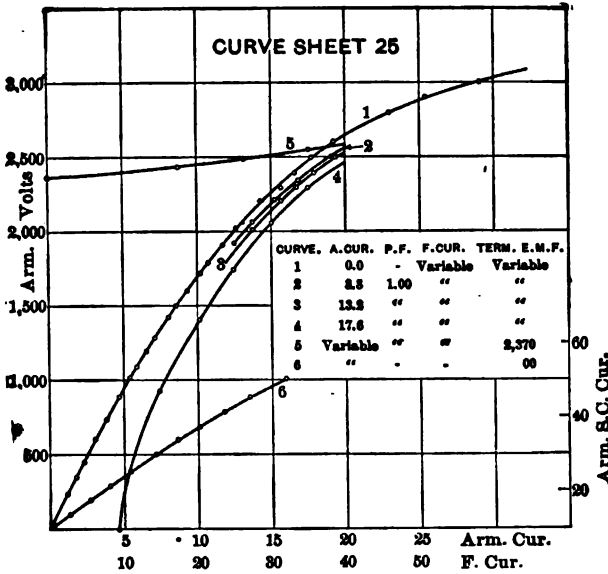
CURVE SHEET 25.—LOAD SATURATION, REGULATION AND SHORT-CIRCUIT CURVES.
