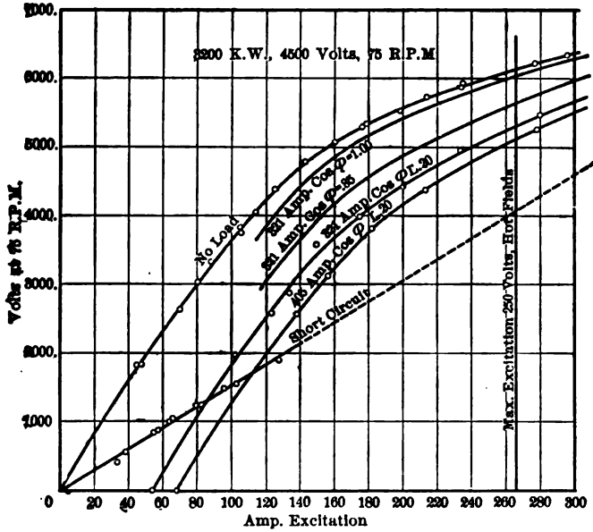
Fig. 10.—REGULATION CURVES ON A 3200-KW ALTERNATOR OBTAINED BY THE AUTHOR'S METHOD.
