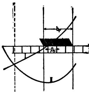
FIG. 15. FIELD AND POTENTIAL CURVE IN THE NEUTRAL ZONE WHEN LOADED.
