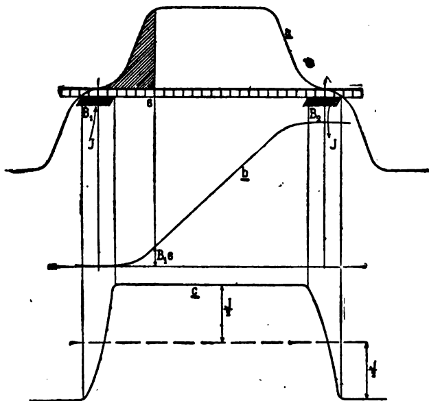
FIG. 2. FIELD POTENTIAL AND CURRENT CURVE OF A CLOSED-CIRCUIT WINDING.
