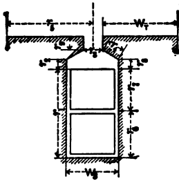
FIG. 1.— SLOT LEAKAGE PATHS.
