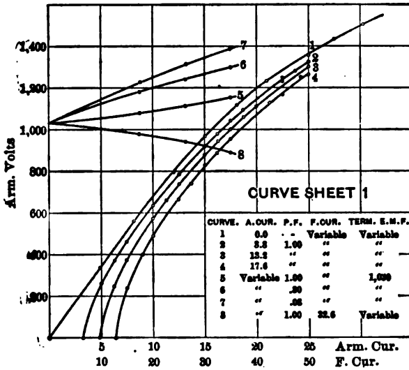
CURVE SHEET 1.—LOAD SATURATION AND REGULATION CURVES. 70 kw, 3-ph, 2300 volts Y. 60 p.p.s., 276 r.p.m., .2525" air-gap.
