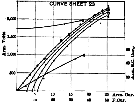
CURVE SHEET 23.—LOAD SATURATION AND SHORT-CIRCUIT CURVES. 70 kw, 3-ph, 2300 volts Y. 60 p.p.s., 276 r.p.m., .2525" air-gap. 2 phase in series.
