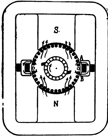
FIG. 42. ARRANGEMENT OF SWINBURNE COMMUTATION POLES.
