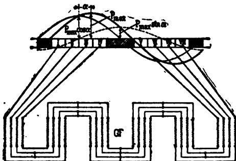
FIG. 58. MEAN POTENTIAL CURVE OF HEYLAND COMMUTATOR.
