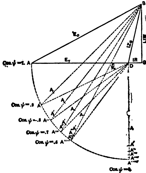
FIG. 6.— REACTANCE METHOD.
