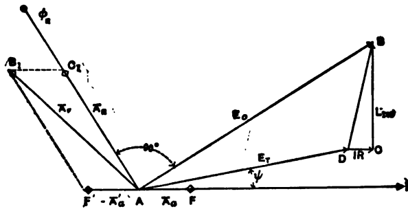
FIG. 4.—GENERAL DIAGRAM.
