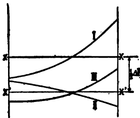
FIG. 5. POTENTIAL CURVE BETWEEN THE NEGATIVE BRUSH OF A GENERATOR AT NO-LOAD (I) AND WHEN LOADED (III).
