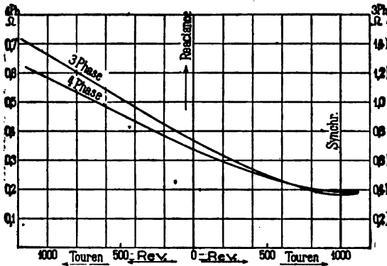
FIG. 53. REACTANCE AS FUNCTION OF REVOLUTIONS.
