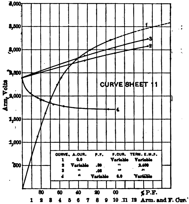
CURVE SHEET 11.— POWER FACTOR LOAD AND SATURATION CURVES. 65 kw, 2-ph, 2400 volts, 60 p.p.s., 900 r.p.m., .0845" air-gap.
