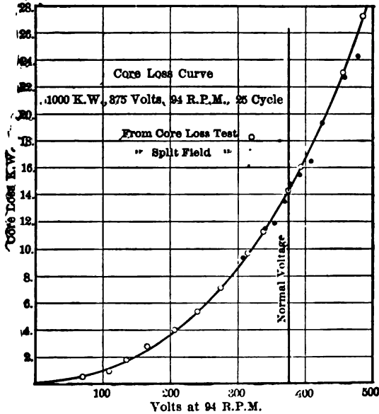
Fig. 11.—COMPARISON OF CORE-LOSSES OBTAINED ON OPEN CIRCUIT AND IN THE AUTHOR'S SPLIT-FIELD TEST.
