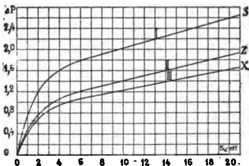
FIG. 8. TRANSITION VOLTAGES OF LE CARBONE CARBONS.
