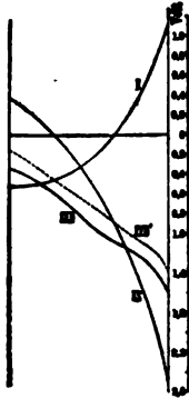
FIG. 28. POTENTIAL CURVES BELOW THE BRUSHES AT NO-LOAD, FOR SHORT-CIRCUIT AND WHEN LOADED.
