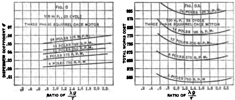
FIGS. 6 AND 6A.—CURVES OF COST RELATION.
