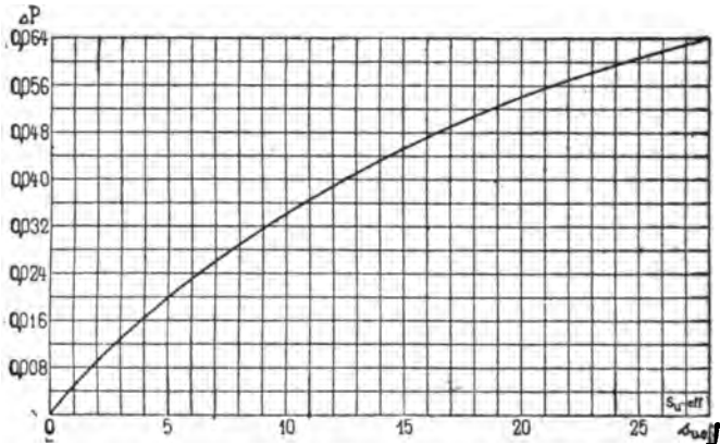
FIG. 9. TRANSITION VOLTAGE FOR COPPER BRUSHES.
