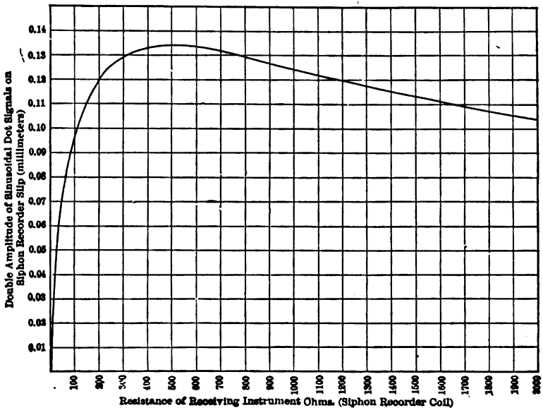
FIG. 8.— DOUBLE AMPLITUDE OF RECEIVED SIGNALS FOR CABLE CONSIDERED WITH +32.14 VOLTS, APPLIED TO SENDING END IN DOTS AND PAUSES, AT FREQUENCY OF 5.78 \sim , WITH VARYING RESISTANCES OF SIPHON RECORDER COIL AT RECEIVING END, THE SENSIBILITY-CONSTANT OF THE INSTRUMENT BEING 400.
