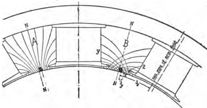
FIG. 14. ARMATURE FIELD OF DIRECT-CURRENT DYNAMO.
