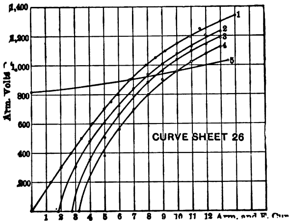
CURVE SHEET 26.—LOAD SATURATION AND REGULATION CURVES.
