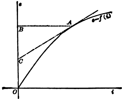
FIG. 1.—OPEN-CIRCUIT CHARACTERISTIC.
