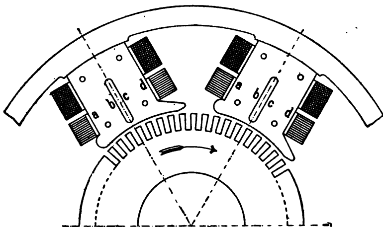
FIG. 43. POLE CONSTRUCTION AND COMPOUND WINDING FOR OBTAINING A STABLE COMMUTATION FIELD.
