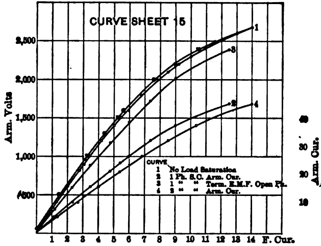
CURVE SHEET 15.—SHORT-CIRCUIT AND SATURATION CURVES. 65 kw, 2-ph, 2400 volts, 60 p.p.s., 900 r.p.m., .280" air-gap.
