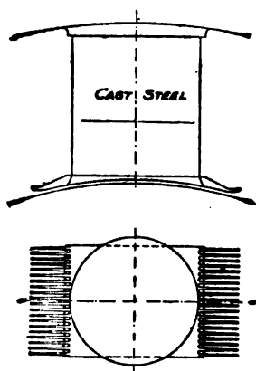
FIG. 37. CAST-STEEL POLE OF GANZ & CO.
