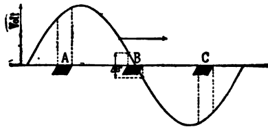
FIG. 46. POTENTIAL CURVE OF THREE-PHASE COMMUTATOR MOTOR.
