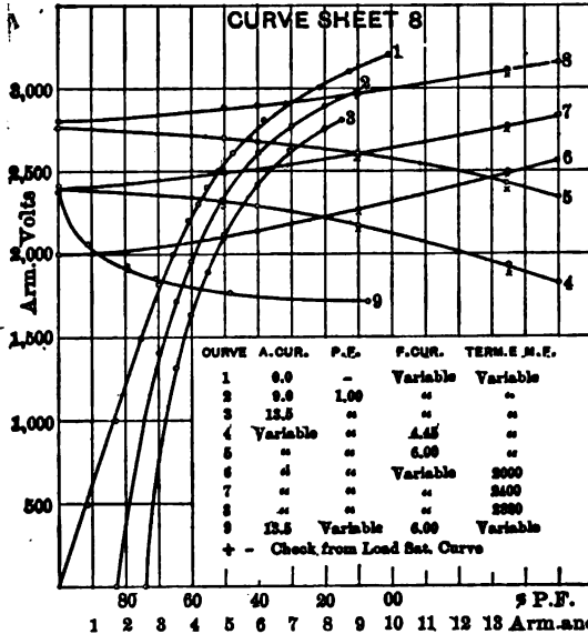
CURVE SHEET 8.—LOAD SATURATION AND REGULATION CURVES. 65 kw, 2-ph, 2400 volts, 60 p.p.s., 900 r.p.m., .0855" air-gap.
