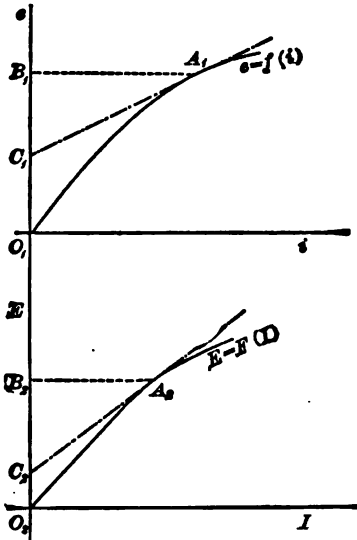
FIG. 2.— CHARACTERISTICS OF ALTERNATOR AND OF EXCITER ON ITS SHAFT.
