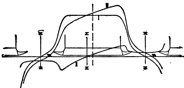
FIG. 3. FIELD CURVES FOR NO-LOAD AND WHEN LOADED.
