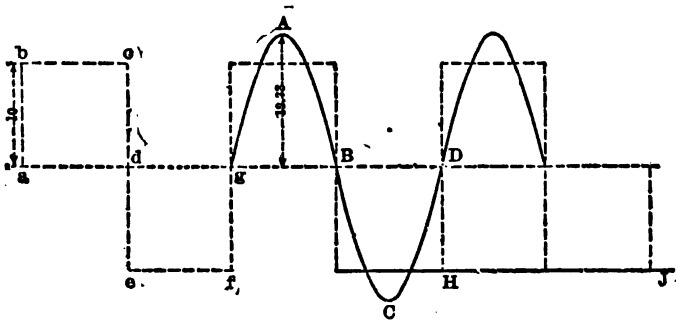
FIG. 2.—DIAGRAM OF RECTANGULAR E.M.F. AND FUNDAMENTAL SINUSOID OF THE SAME.
