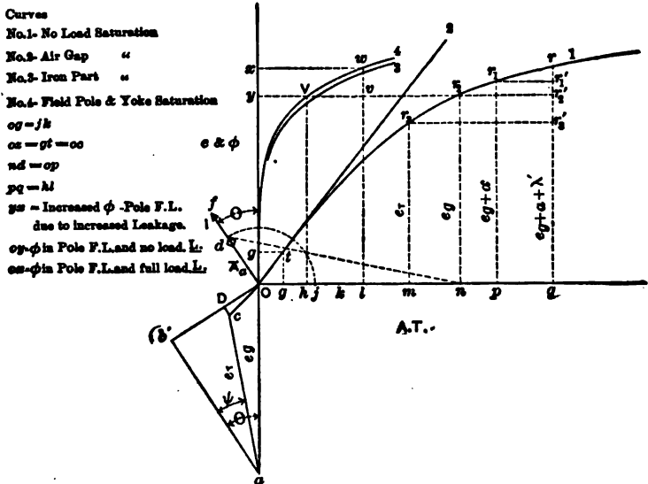
FIG. 2.— COMPLETE GENERAL DIAGRAM.
