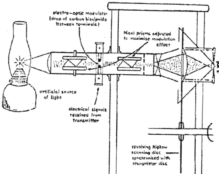
Schematic of Sutton's Telephone (designed 1885)
