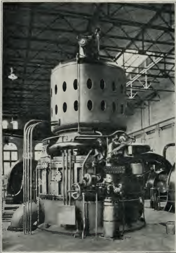
2000 K. W. STEAM TURBINE, POTOMAC ELECTRIC POWER CO.
