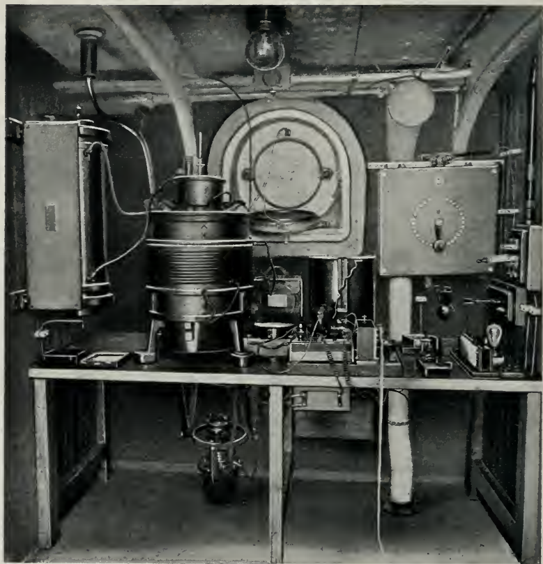
OPERATING ROOM, WIRELESS TELEGRAPH Fig. 1.
