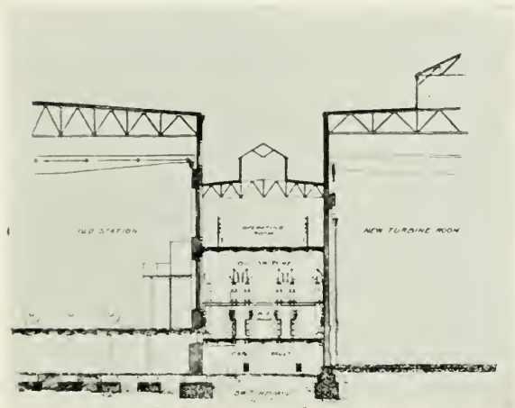
Section, I. Street Station
