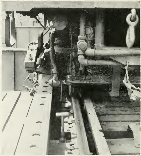
Automatic Stop for Air-brakes
