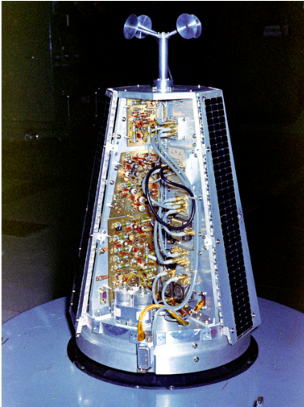
Small Satellite A developed by NHK (10kg)
